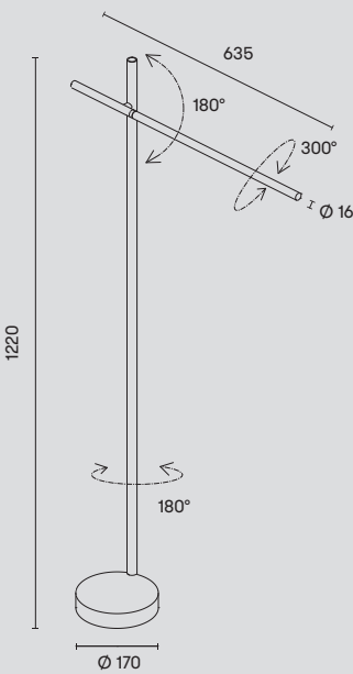
25-8102-05-M1 (Touch dimming) LED 10.5W A++ A 1134 lm 3000K
