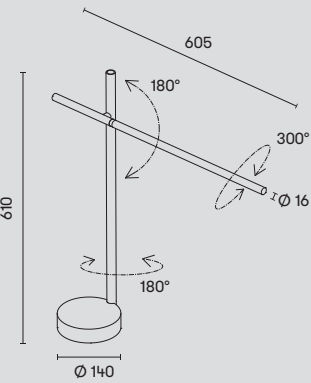
10-8102-05-M1 (Touch dimming) LED 10.5W A++ A 1134 lm 3000K
