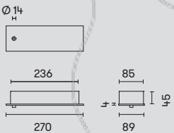
71-8265-05-05 176-305V Max. 105W
